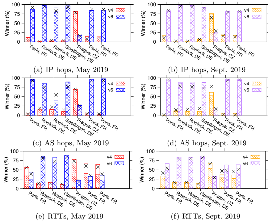
Fig. 5. Differences in the fraction of instances that the IPv6 path (blue/purple) and IPv4 path (red/orange) is the winner, as broken down per PlanetLab node
