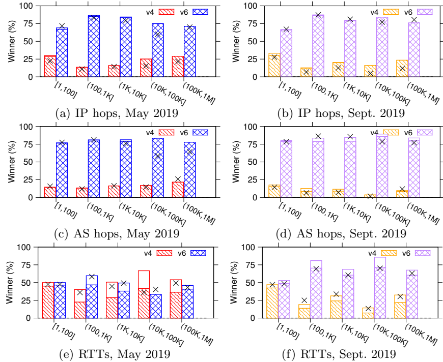
Fig. 3. Fraction of instances that the IPv6 path (blue/purple) and IPv4 path (red/orange) is the winner, as broken down per the rank of the top-1M domains
