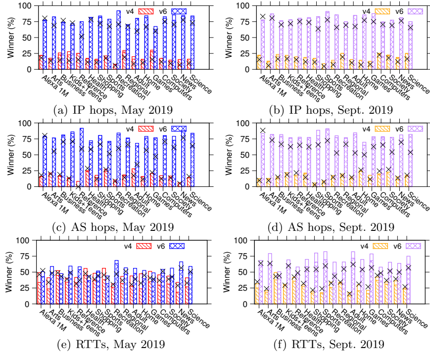
Fig. 4. Fraction of instances that the IPv6 path (blue/purple) and IPv4 path (red/orange) is the winner, as broken down per the domain category
